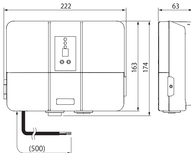
75W 12V HEA-019I/G
