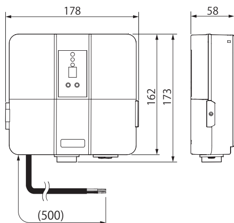
35W 12V HEA-018I/G
